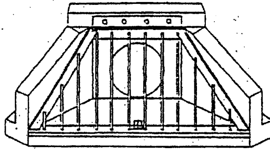
ISOMETRIC
